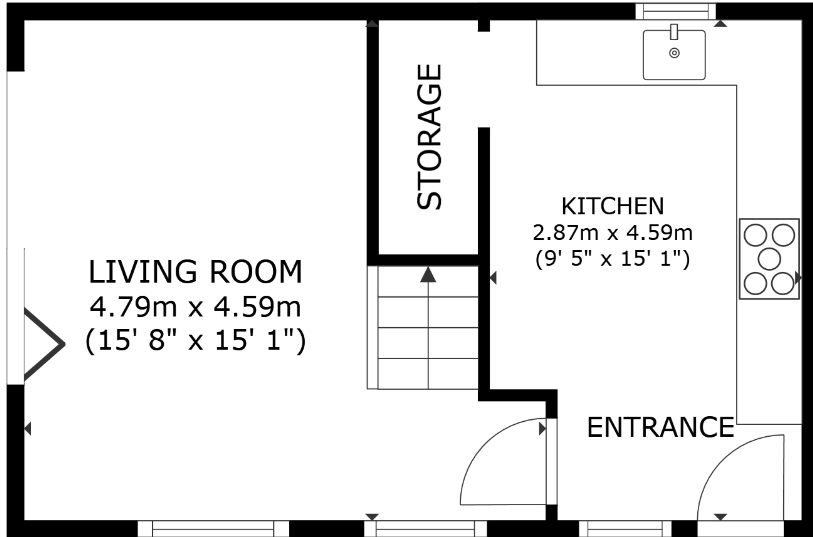
FLOOR 1
